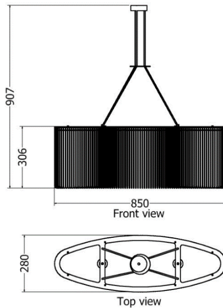
Model LDF-CL-803030v1
