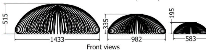
Models LDF-CL-15010, 10010, 1005
